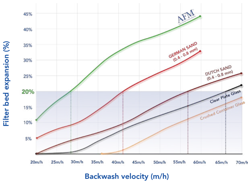
Filter bed expansion at 25°C
